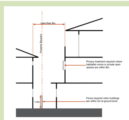
Habitable room windows, balconies, terraces, decks and patios should be designed and located to avoid direct views into secluded private open space and habitable windows of existing dwellings, within a horizontal distance of 9m.
